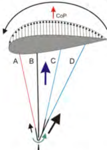
Automatic compensation of SRS
